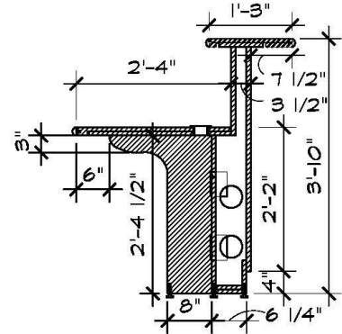
SUPPORT B (FOR USE WITHIN A WORKSTATION OF SEATED HEIGHT)
